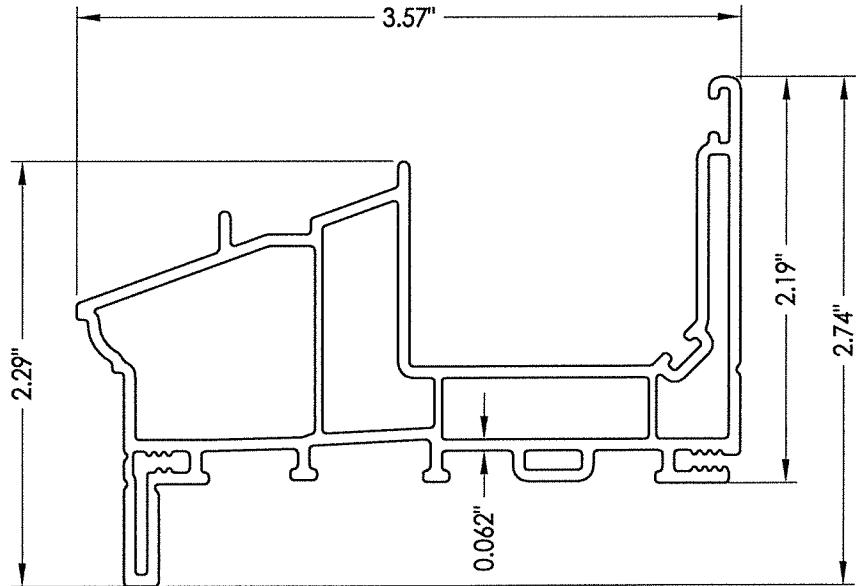
4 SILL
