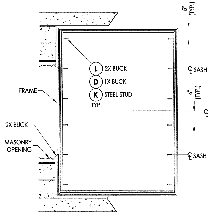
FRAME ANCHORING ALTERNATE ANCHORING (SEE SHEET 3) (MAX. D.P. = 50 PSF)
